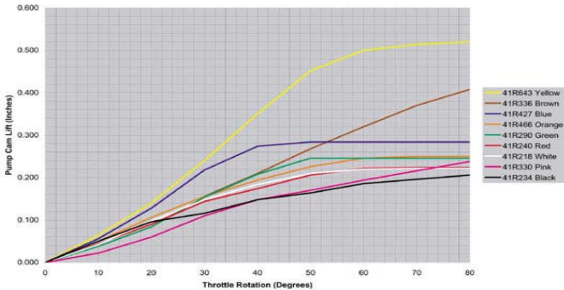
Pump Cam Lift vs. Throttle Position
